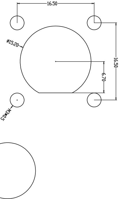
Recommended Panel Cut-out
